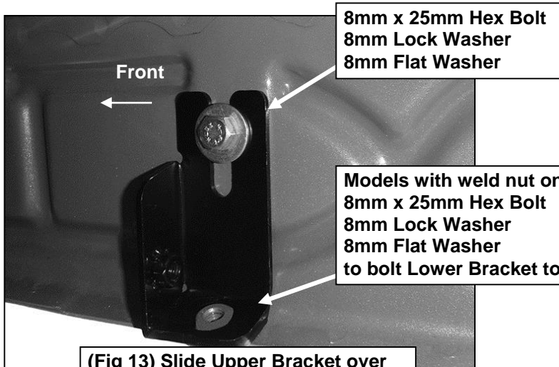
(Fig 13) Slide Upper Bracket over weld nut (if equipped-see Figure 2)
